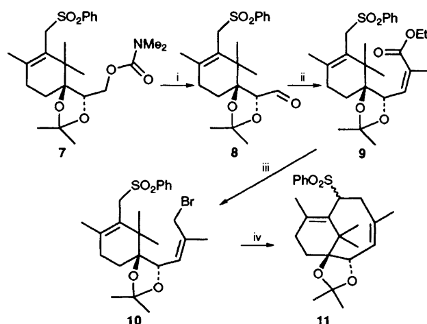
Scheme 2 Reagents and conditions: i, \text{KOH} , \text{MeOH} , 83% then TPAP, \text{NMO} , 89%; ii, (\text{CF}_3\text{CH}_2\text{O})_2\text{P(O)CHMeCO}_2\text{Et} , \text{KHMDS} , 18-crown-6, -78^\circ\text{C} , 52%; iii, Dibal-H, 73% then \text{PPh}_3 , \text{CBr}_4 , 60%; iv, \text{LiHMDS} , 0^\circ\text{C} , 88%
